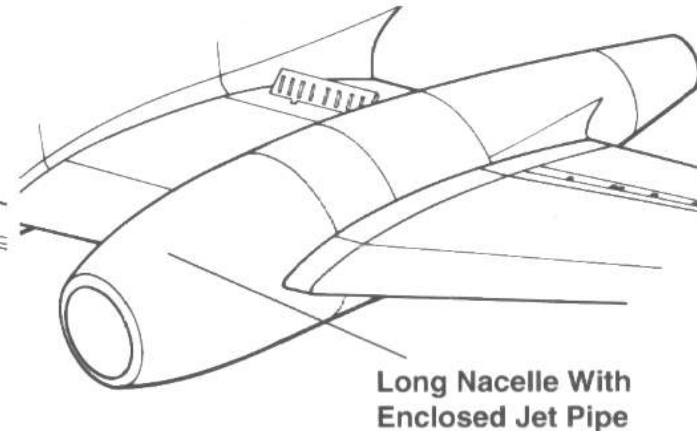
Meteor F 4
